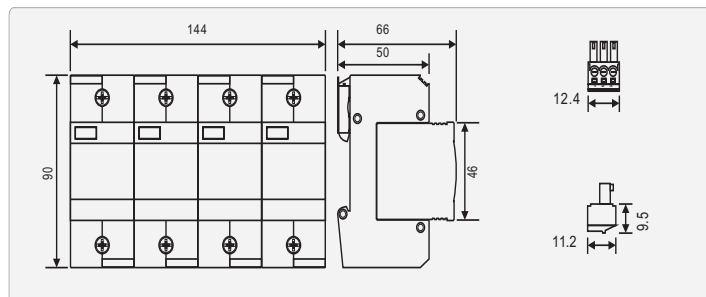
BT P BCM 25 RM/4P Dimension diagram
