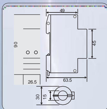
IC03/ IC04_Dimension diagram
